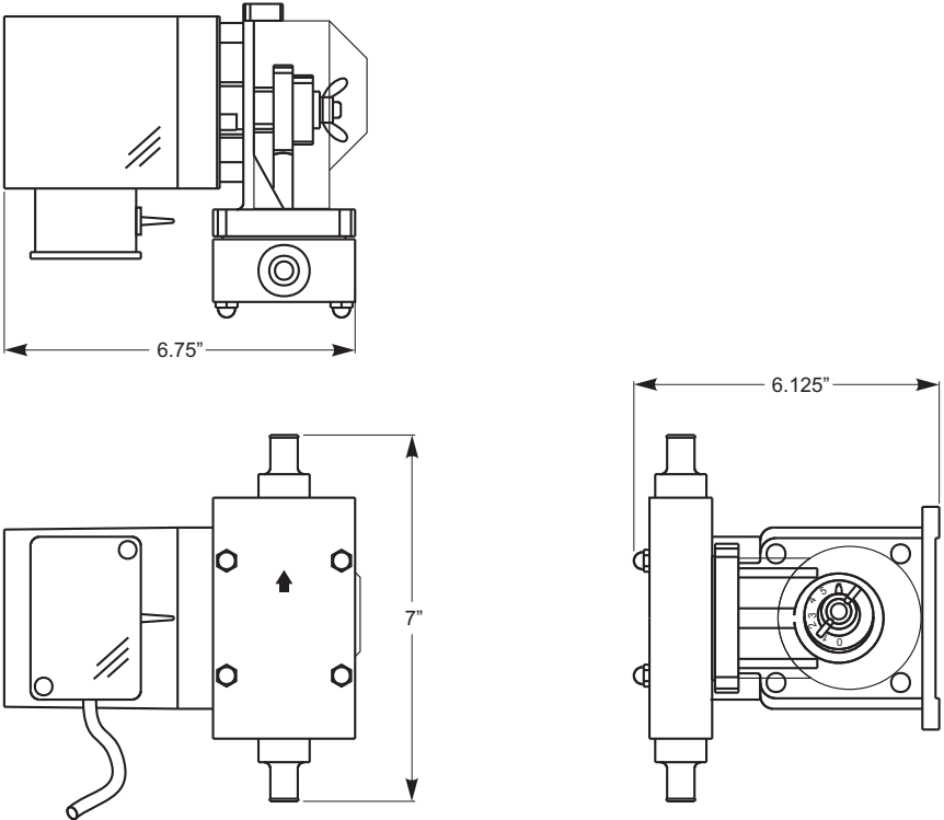
FIG. 4.1 DIMENSIONAL DRAWING
